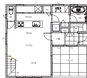
1F
